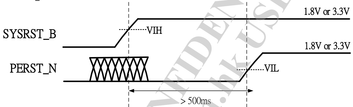
Figure 4 PERST_N sequence
